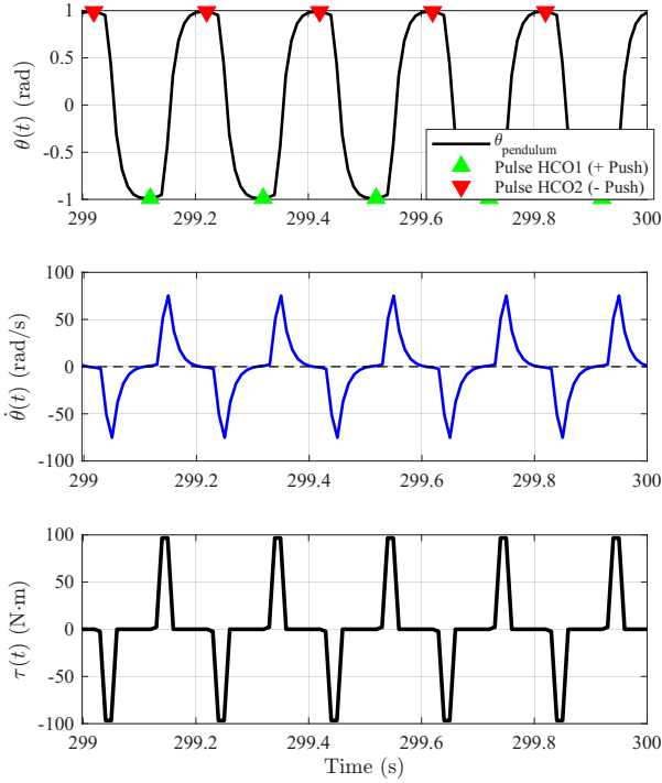
Fig. S5. Steady-state closed-loop dynamics ( t = 299 to 300 s). (Top) Pendulum angle \theta . (Middle) Angular velocity \dot{\theta} . (Bottom) Event-triggered feedback modulation injected at the mechanical extrema ( \dot{\theta} = 0 ) to dynamically synchronize the oscillator phase with the physical plant.
